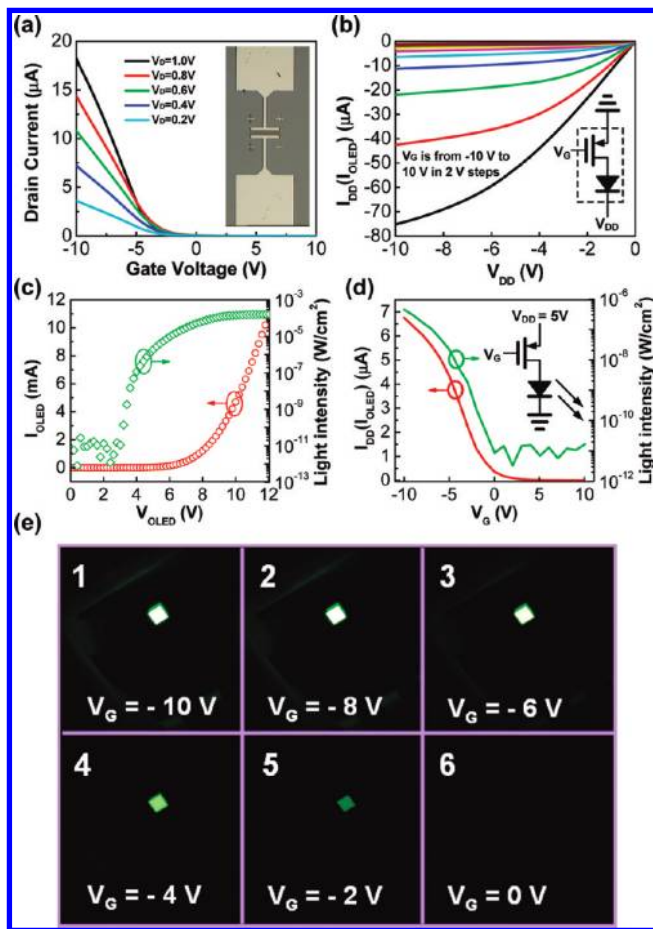
Figure 5. OLED control circuit by SN-TFT. (a) Transfer ( I_D – V_G ) characteristics under different drain voltages for the device used to control the OLED ( L = 20 \mu\text{m} , and W = 100 \mu\text{m} ), Inset: optical microscope image of the device. (b) Characteristics of the OLED control circuit where the current flow through the OLED ( I_{\text{OLED}} ) is measured by sweeping the V_{\text{DD}} and Input voltage V_G . Various curves correspond to various values of V_G from -10 to 10 V in 2 V steps. (c) Two terminal measurement of the OLED showing the current through the OLED ( I_{\text{OLED}} ) (red line) and OLED light intensity (green line) versus the voltage applied across the OLED ( V_{\text{OLED}} ). (d) Plot of the current through the OLED ( I_{\text{OLED}} ) (red line) and OLED light intensity (green line) versus V_G with V_{\text{DD}} = 5 V. Inset: The circuit diagram of an OLED driven by a SN-TFT. (e) Photographs of the OLED driven by SN-TFT under different inputs showing the turn on and turn off of the OLED.
