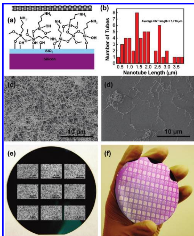
Figure 1. Wafer-scale deposition of separated carbon nanotubes and fabrication of SN-TFTs. (a) Schematic diagram of APTES assisted nanotube deposition on Si/SiO 2 substrate. (b) Length distribution of the separated nanotubes used in this study; the average nanotube length is 1.716 \mu\text{m} . (c, d) FE-SEM images of separated nanotubes deposited on Si/SiO 2 substrates with (c) and without (d) APTES functionalization, respectively. (e) Photograph of 3 in. Si/SiO 2 wafer after APTES assisted nanotubes deposition. Inset: FE-SEM images showing nanotubes deposited at different locations on the wafer, the locations of the SEM images on the wafer correspond to the approximate locations on the wafer where the images were taken. All the scale bars are 5 \mu\text{m} . (f) Photograph of the same wafer after electrode patterning. The wafer consists of SN-TFTs used in this study and other types of electronic devices. Such SN-TFTs are made with channel width ( W ) of 10, 20, 50, 100, and 200 \mu\text{m} , and channel length ( L ) of 4, 10, 20, 50, and 100 \mu\text{m} .
