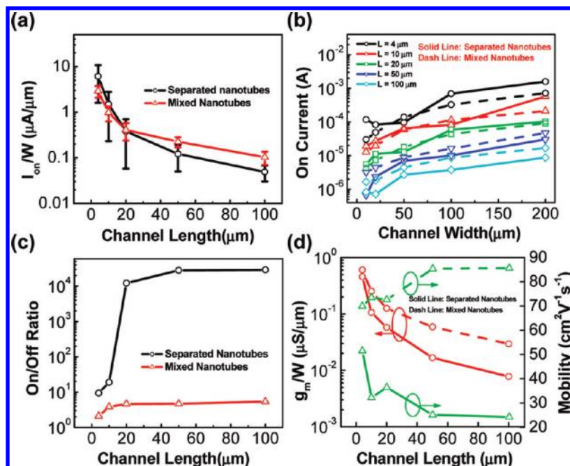
Figure 3. Statistical study of 200 nanotube TFTs based on separated nanotubes and mixed nanotubes. (a) Plot of current density ( I_{on}/W ) versus channel length for TFTs fabricated on separated nanotubes and mixed nanotubes. (b) Plot of average on current ( I_{on} ) versus channel width for TFTs fabricated on separated nanotubes and mixed nanotubes with various channel lengths (4, 10, 20, 50, 100 \mu m ). (c) Plot of average on/off ratio ( I_{on}/I_{off} ) versus channel length for TFTs fabricated on separated nanotubes and mixed nanotubes. (d) Plot of average transconductance per unit width ( g_m/W ) and average device mobility ( \mu_{device} ) versus channel length for TFTs fabricated on separated nanotubes and mixed nanotubes.
