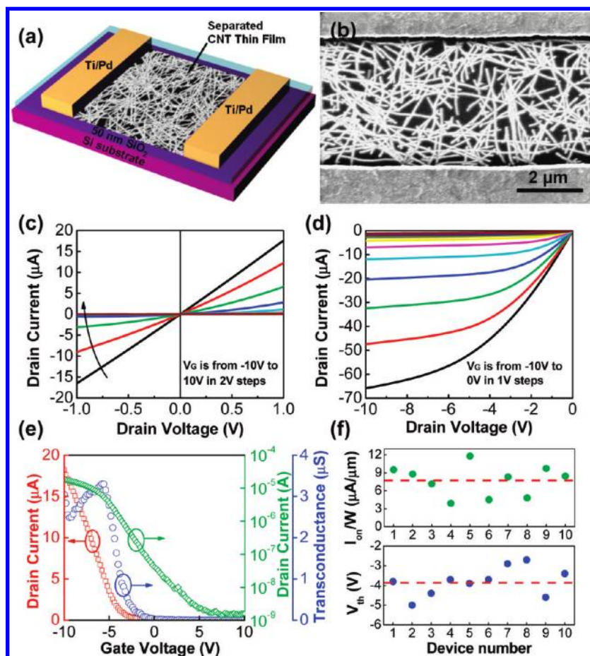
Figure 2. Electronic properties of back-gated SN-TFTs. (a) Schematic diagram of a back-gated transistor built on separated nanotube thin-film with Ti/Pd (5 Å/70 nm) contacts and SiO 2 (50 nm) gate dielectric. (b) FE-SEM image of a typical SN-TFT with 4 μm channel length. (c,d) Output ( I_D-V_D ) characteristics of a typical SN-TFT ( L = 20 \mu\text{m} and W = 100 \mu\text{m} ) in triode region (c) and saturation region (d), respectively. (e) Transfer ( I_D-V_G ) characteristics (red, linear scale; green, log scale) and g_m-V_G characteristics (blue) of the same device with V_D = 1 \text{ V} . (f) Current density ( I_{\text{on}}/W ) measured at V_D = 1 \text{ V} and threshold voltage ( V_{\text{th}} ) of 10 representative SN-TFTs showing the uniformity of devices. The red line represents the average value.
