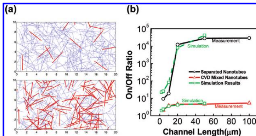
Figure 4. Simulation of nanotube thin-film percolation network. (a) Randomly generated nanotube percolation networks of separated nanotubes (top) and mixed nanotubes (bottom) for devices with L = 10 \mu\text{m} and W = 20 \mu\text{m} . The red and blue lines represent metallic and semiconductive nanotubes, respectively. (b) Comparison between the simulation data derived from the percolation network and measurement data.
